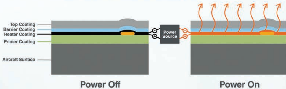
Battelle's powered nano-coating prevents ice build-up on critical aerospace surfaces.
